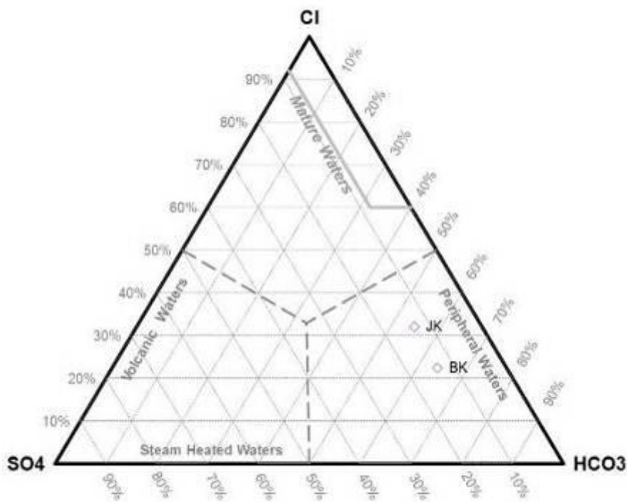
Figure 7. The result of plot of water chemistry data of Pandan volcano area on Cl-HCO 3 -SO 4 diagram. The sample of the research area is located on the peripheral water area
